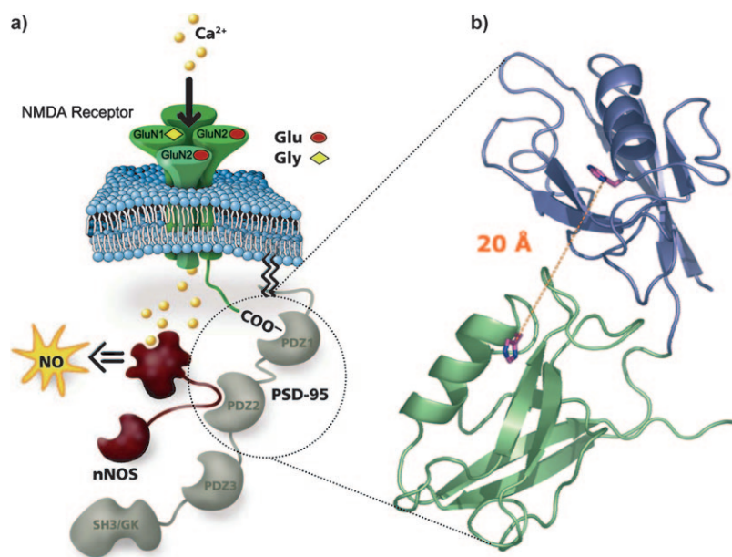
Figure 1. a) PSD-95 facilitates \text{Ca}^{2+} -mediated excessive NO production during excitotoxicity, which can be impaired by inhibition of the PSD-95–NMDA receptor interaction. b) Structural model of PDZ1-2, where two conserved histidine residues, important for ligand binding, and their relative distance are highlighted. [11] SH3/GK = src homology 3/ guanylate kinase; src proteins cause sarcomas.
